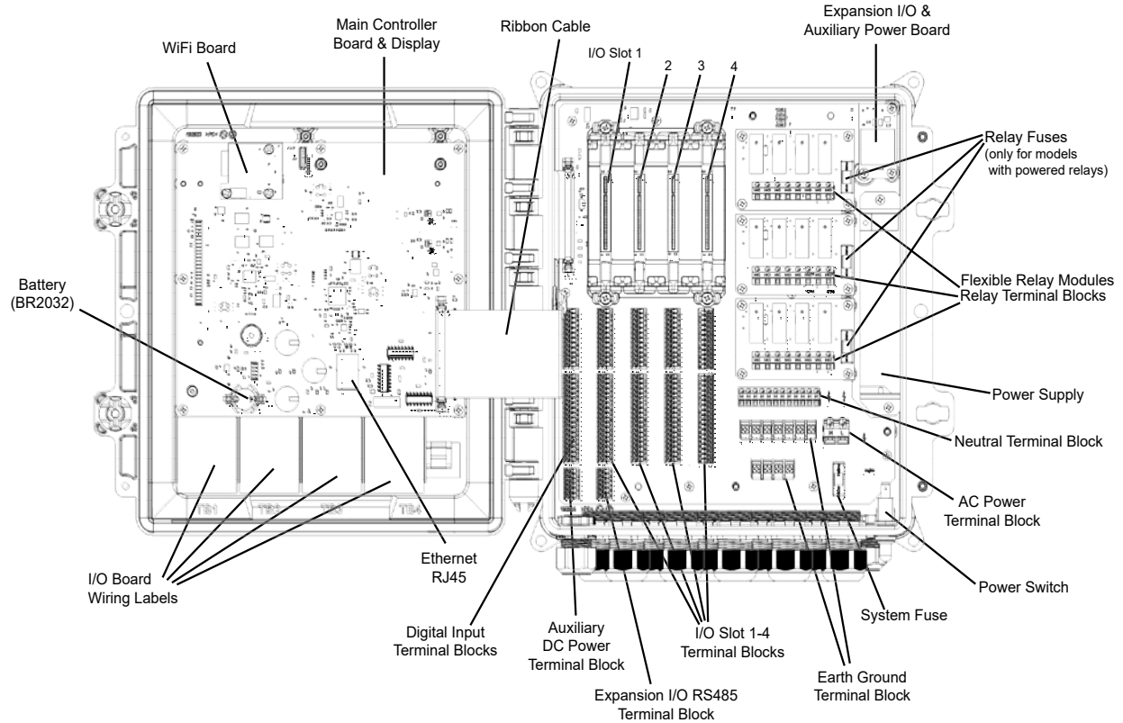
Figure 6 Parts Identification
